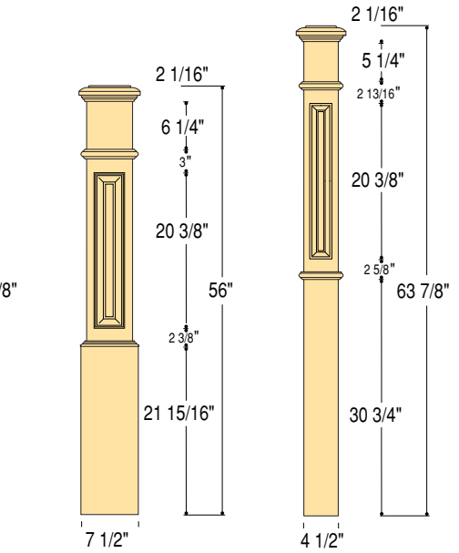
C-4891-RP True Raised Panel 6" Top Sq. 7 1/2" Bottom Sq.
