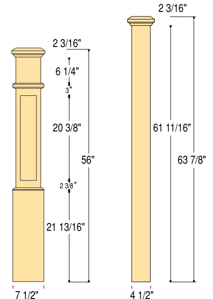
C-4890 Mission 6" Top Sq. 7 1/2" Bottom Sq.
