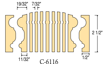
C-6116 Bending Rail with Bending Mould
