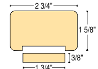
C-6700 P1 with Fillet
