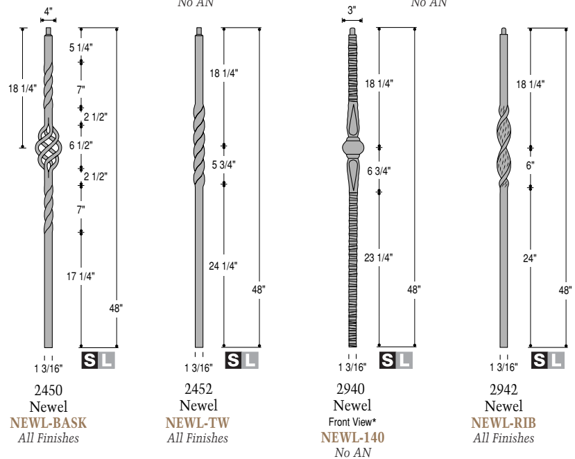
Shown: Detail 2450 Newel
