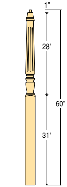
C-4275 3 1/2" Sq. Flute Intermediate or Landing
