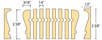
C-6216 Bending Rail with Bending Mould
