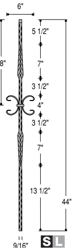
2998 Front View M120 All Finishes (No AN - Solid)
