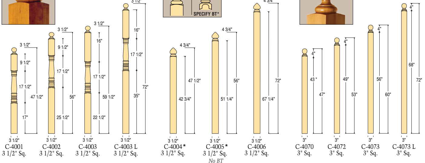
Newel Top Detail
