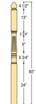
C-4285 3 1/2" Sq. Flute
