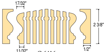
C-6416 Bending Rail with Bending Mould
