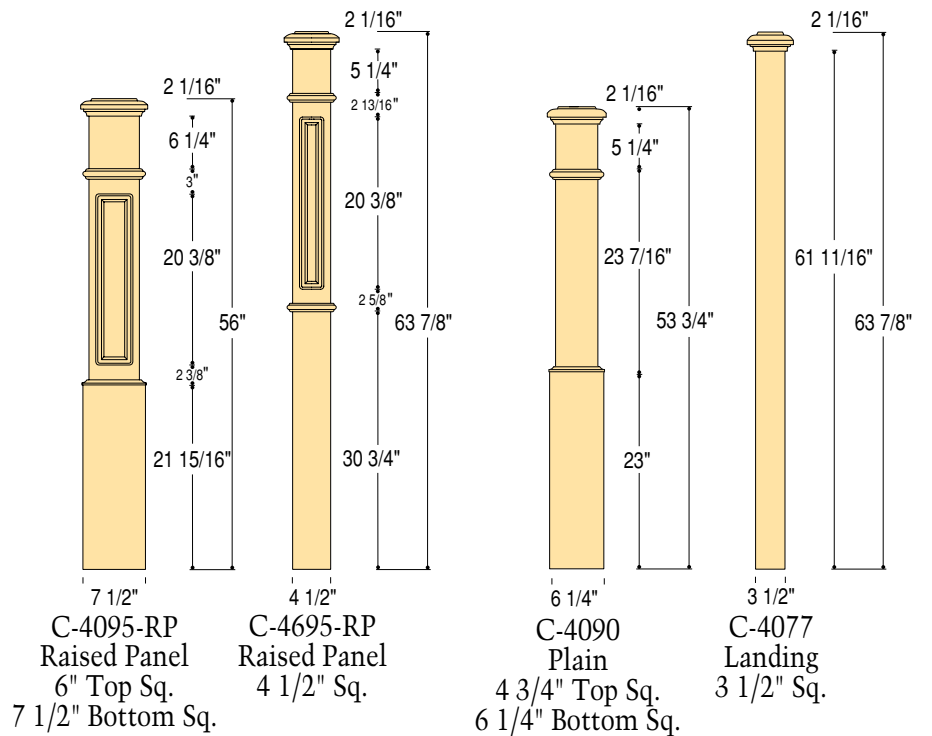
Shown: C-4695-RP Raised Panel Box Newel
