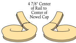
4 7/8" Center of Rail to Center of Newel Cap C-7030 C-7035 C-7230 C-7235 Left Hand Volute Right Hand Volute
