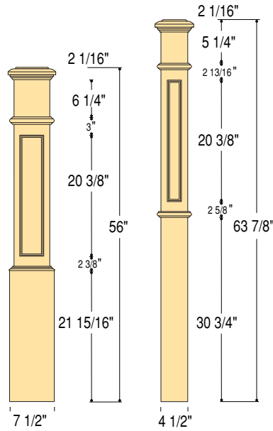
C-4891-FP Flat Panel 6" Top Sq. 7 1/2" Bottom Sq.
