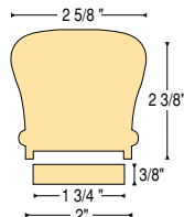
C-6210 P1 with Fillet
