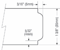
Sticking Profile
