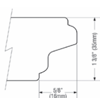
Rail Profile
