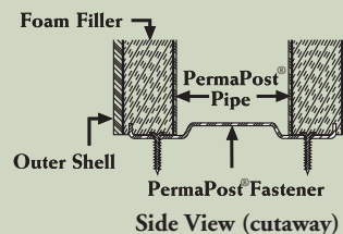
Side View (cutaway)
